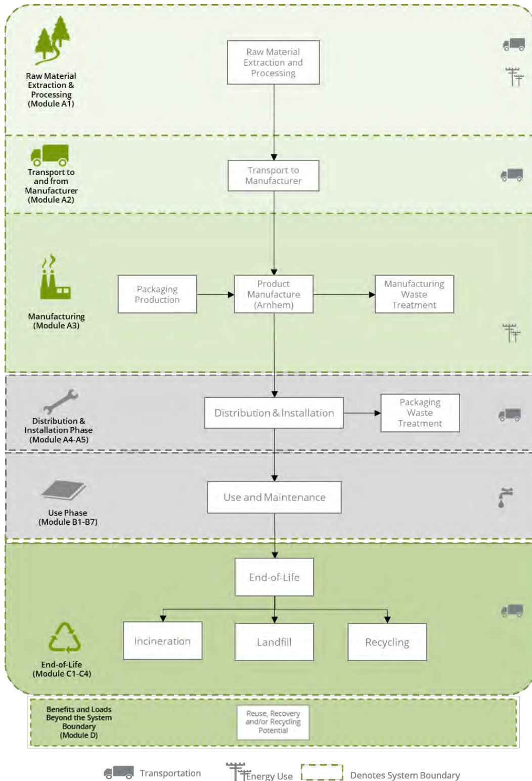
Figure 2. Flow diagram and system boundaries for the life cycle of the Accoya Wood products produced at Arnhem.
